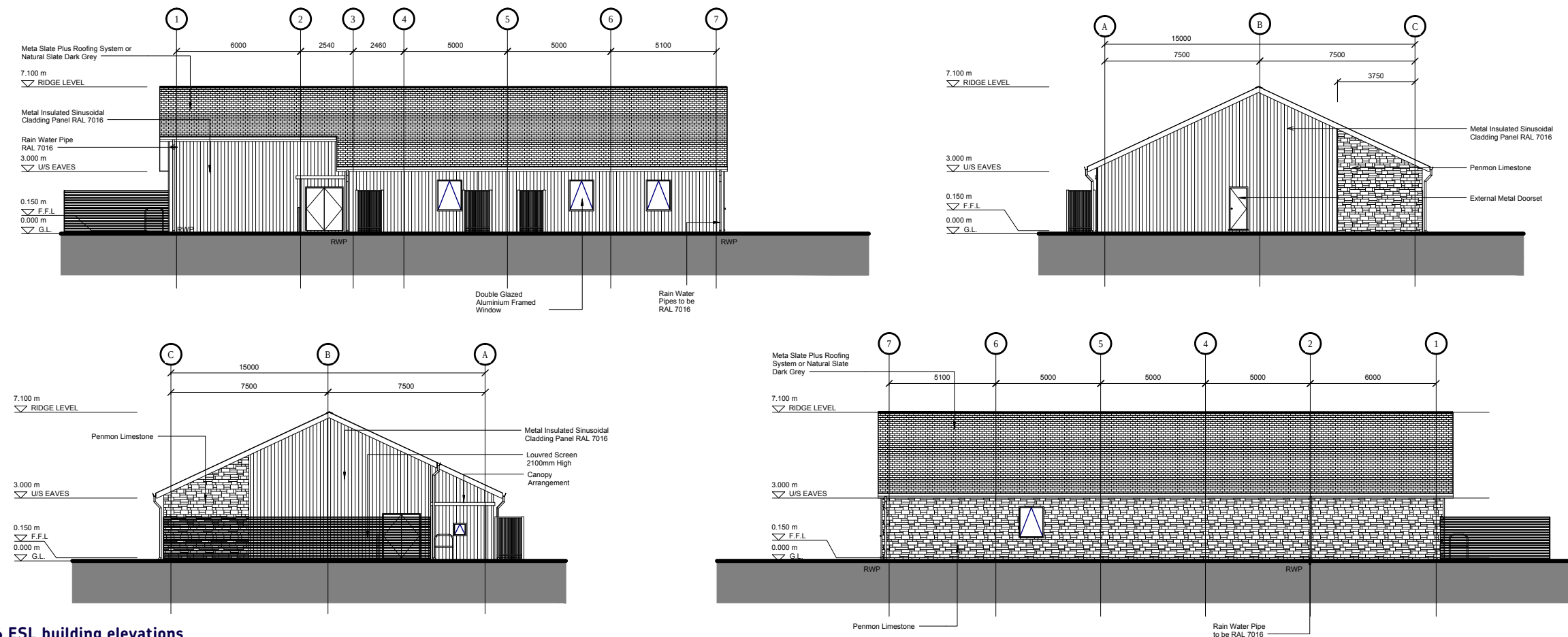
Figure 36 ESL building elevations
